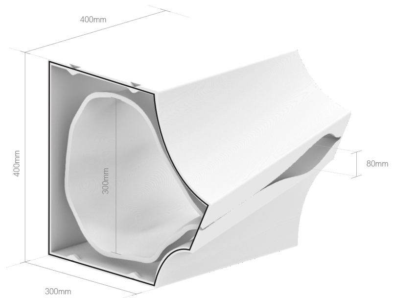
Isometric Jackdaw Nest Tile
