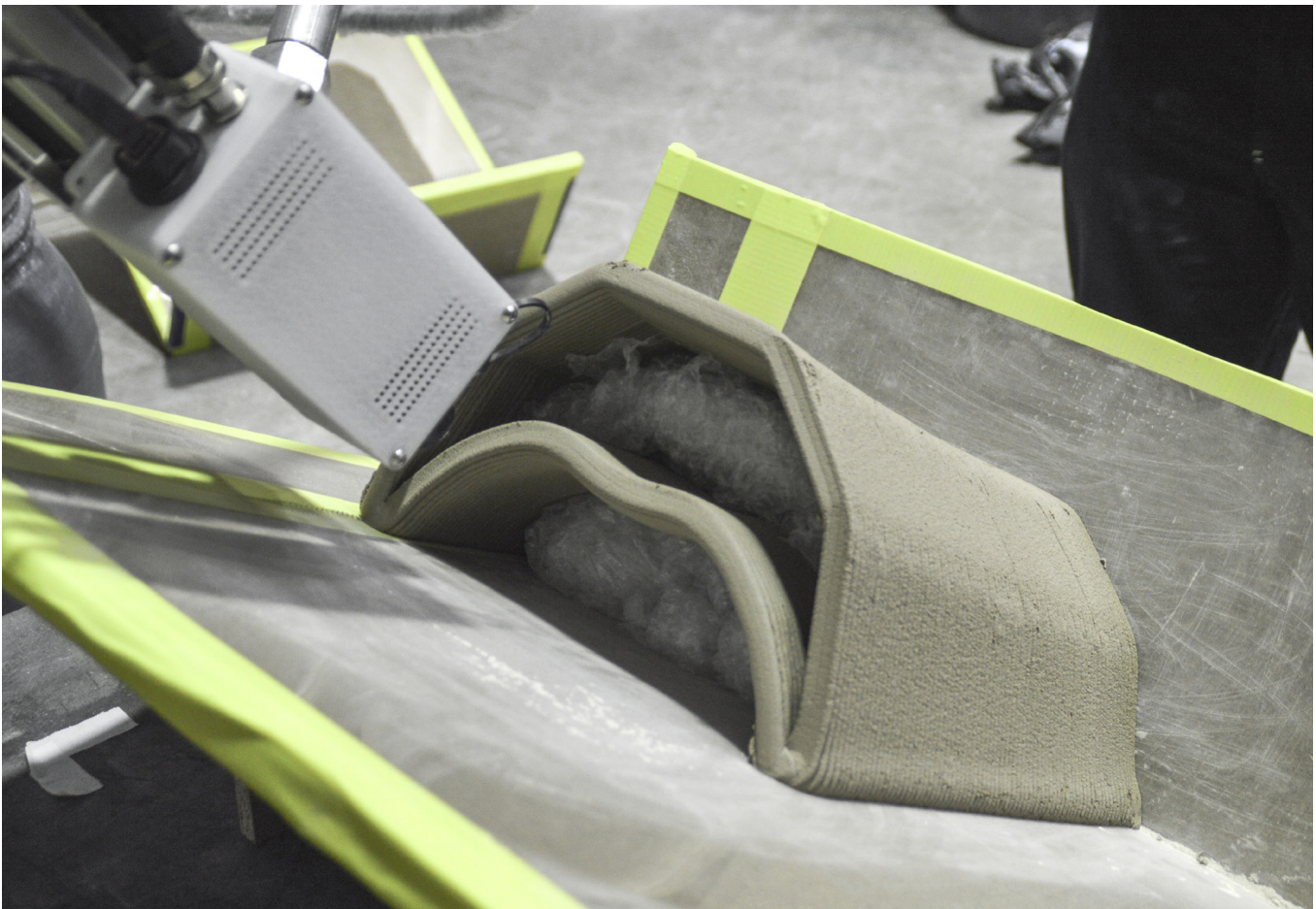
Printing with substructure 30 degree | Nest element
