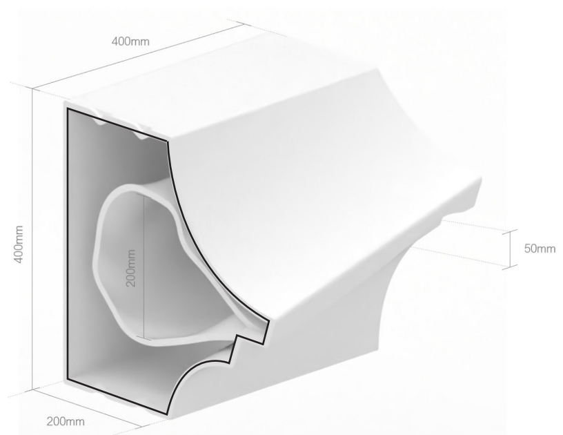
Isometric Black Redstart Nest Tile
