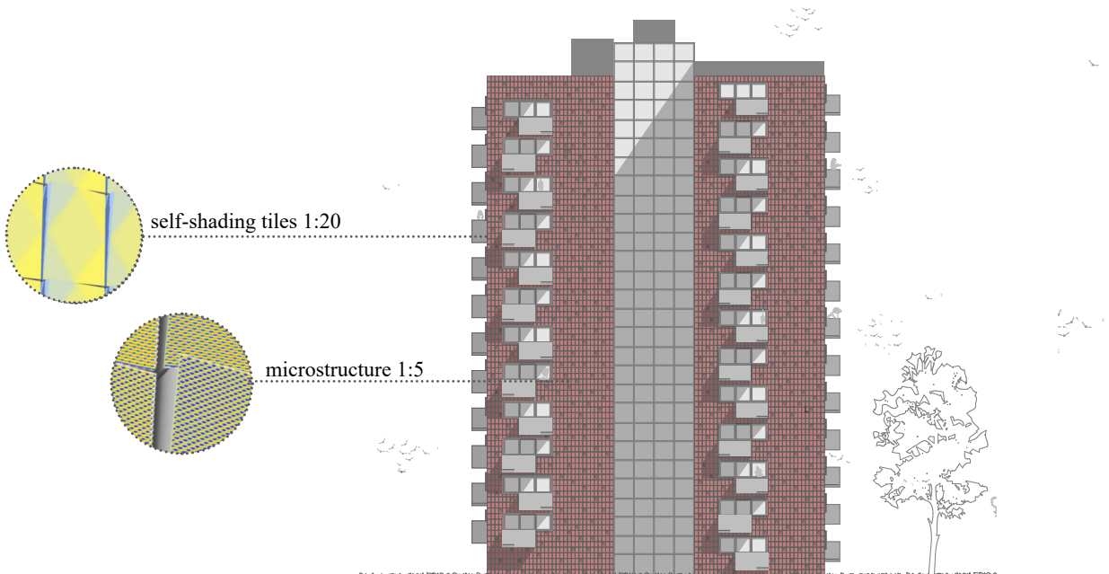
Elevation South Facade Brückenkopf 8, 85051 Ingolstadt
