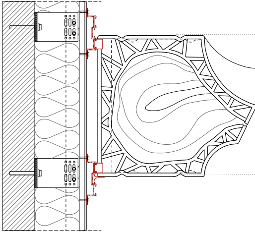
Section 1:20
