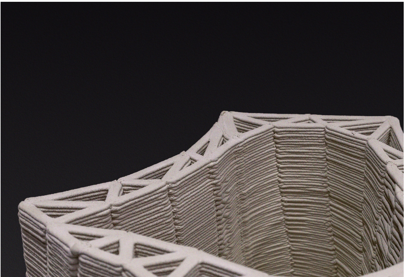
Detail of support structure which simultaneously forms inner and outer shell.
